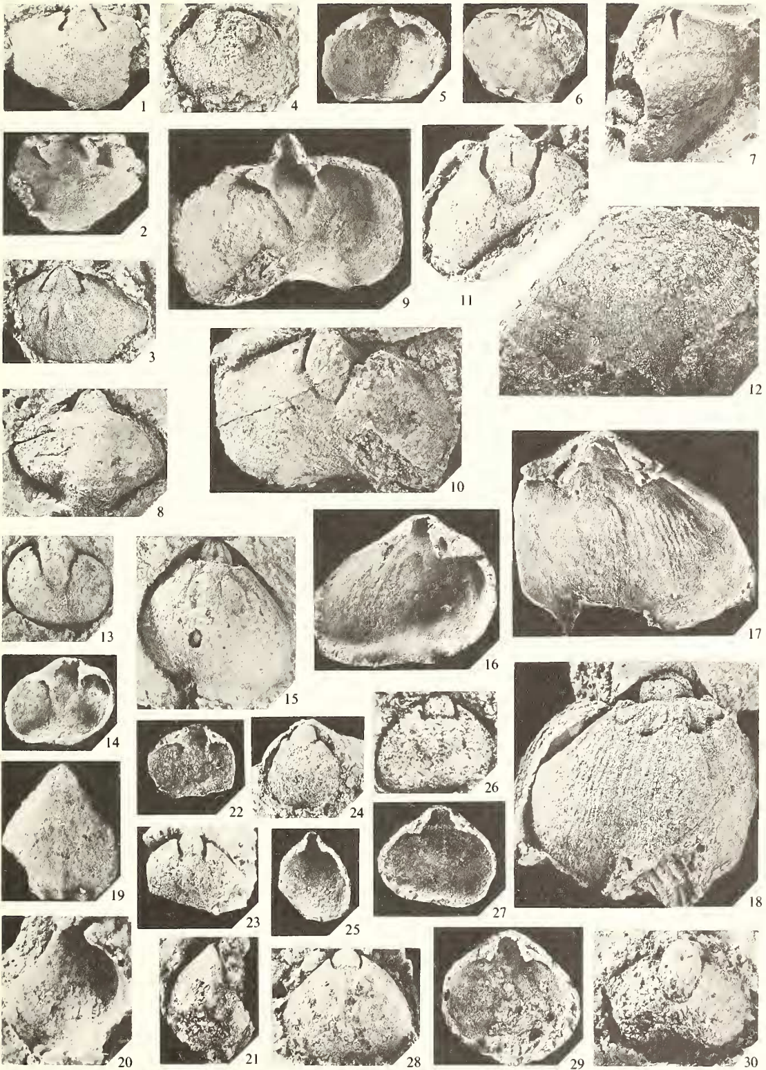
NEUMAN and BATES, early Ordovician brachiopods
